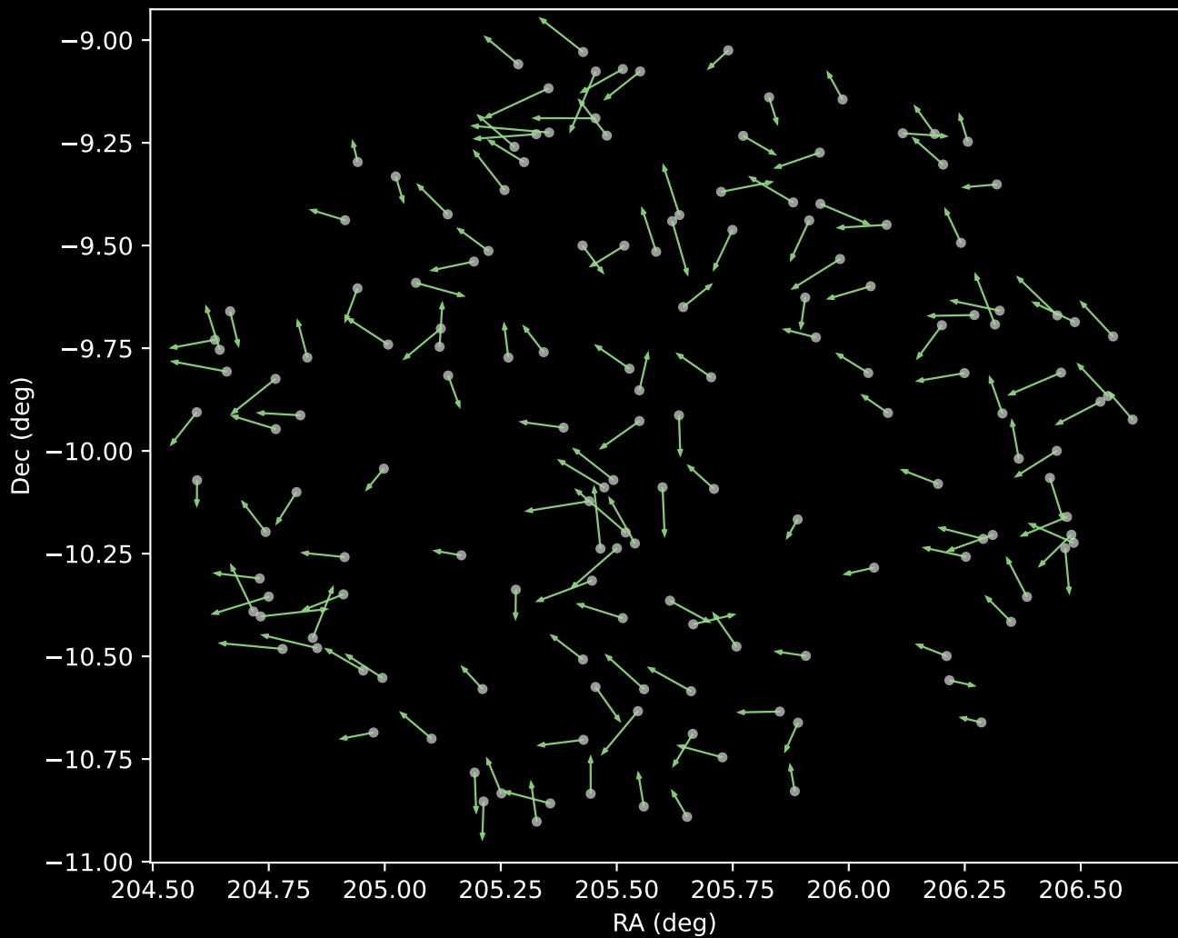
GALAH DR4 Cluster 5 Proper Motion Vectors (n=156)
