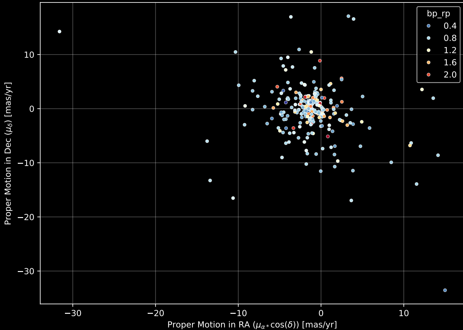
GALAH DR4 Field: [8896] Proper Motion Diagram (n= 260)
