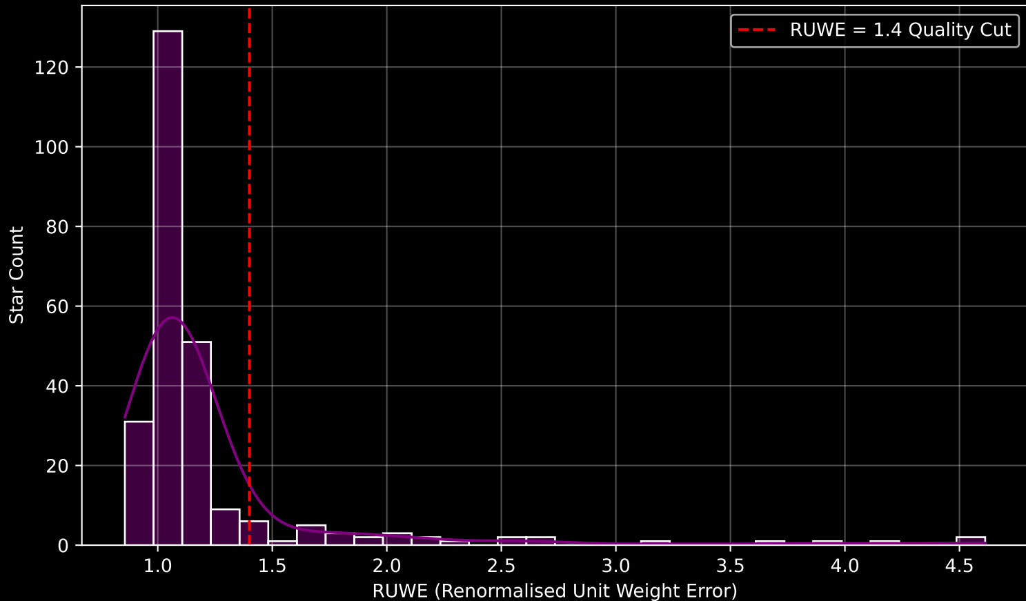
GALAH DR4 Field [8896] RUWE Distribution (n= 253)
