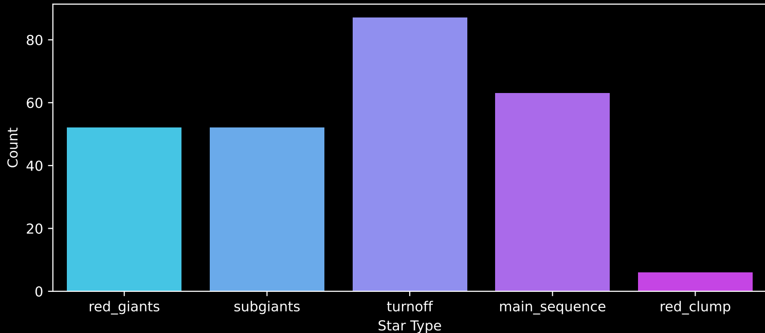
GALAH DR4 Field: [8896] Count plot of Star Type
